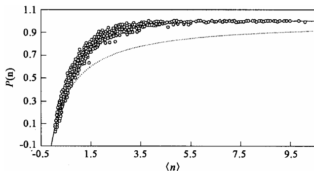
Fig. 8—Distribution of P(n) form Lampyridae (measured parameters: \Delta t=0.1s , \Delta\tau=10^{-4}s , \tau=10^{-5}s )
