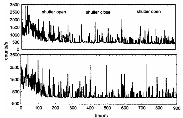
Fig. 7—Synchronous flickering of Dinoflagellates. Gonyaulax
