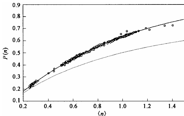
Fig. 2—Measured P(n) from Denoflagellate eleganece (measured parameters: \Delta t=1 s, \Delta\tau = 3 \times 10^{-4} s, \tau \approx 10^{-7} s)
