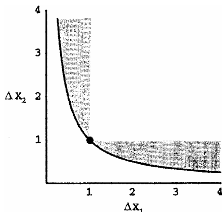
Fig. 6—Heisenberg's uncertainty principle. (Walls and Milburn, 1994, Quantum Optics )
