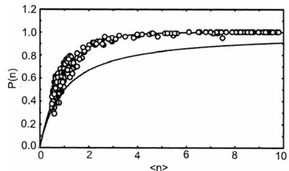
Fig. 5—Measured P(n) from Denoflagellate eleganece (measured parameters: \Delta t=1 s, \Delta\tau = 10^{-3} s, \tau \approx 10^{-7} s.)
