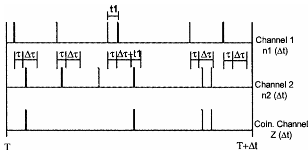
Fig. 1—The principle of coincidence counting system
