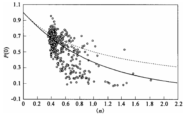
Fig. 3—Measured P(0) from Denoflagellate gonyaulax (measured parameters: \Delta t=1 s, \Delta\tau = 3 \times 10^{-3} s, \tau = 10^{-5} s)
