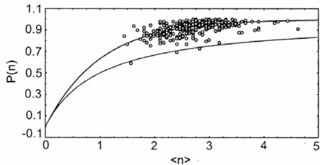
Fig. 4—Measured P(n) from brains of chicken embryos (measured parameters: \Delta t=1 s, \Delta\tau = 6 \times 10^{-2} s, \tau \approx 10^{-7} s.)
