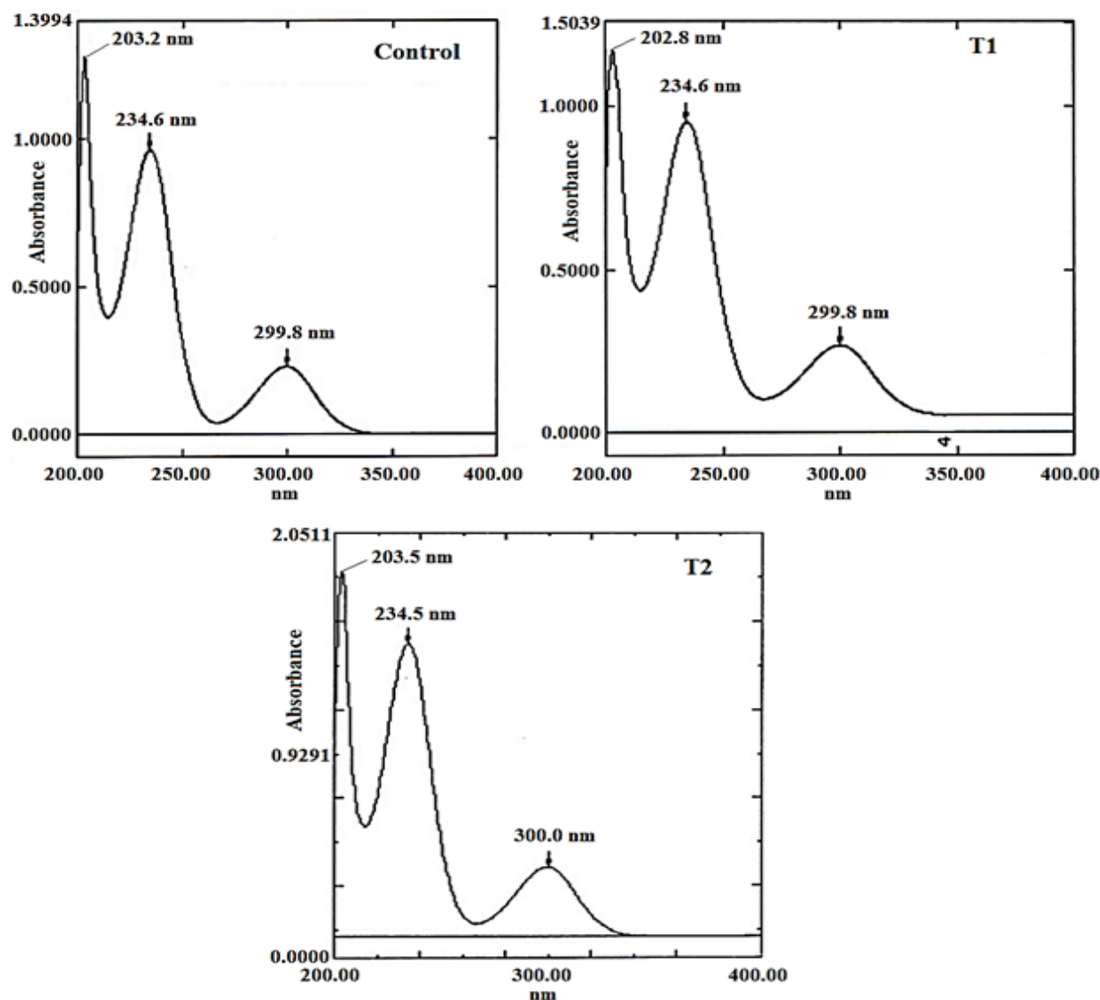
Figure 6: UV-Vis spectra of control and treated (T1 and T2) p -anisidine.
