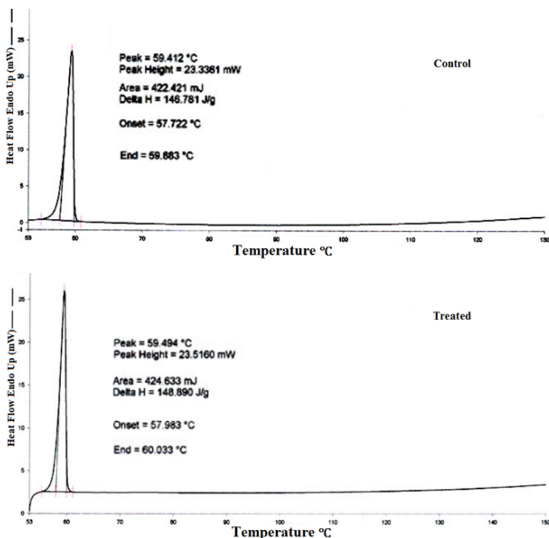
Figure 3: DSC thermogram of control and treated p -anisidine.
