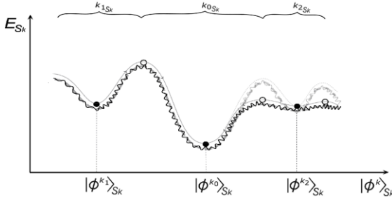
Fig. 1. Schematic presentation of the adaptation of memory attractors in the energy-state hypersurface of the quantum-holographic memory/propagator of various hierarchical levels of biological macroscopic open quantum systems S_k (cellular biomolecular protein/ target, acupuncture system/ consciousness, or out-of-body consciousness/ collective consciousness) [6-19]. It should be pointed out that Nature presumably has chosen elegant room-temperature solution for quantum-holographic information processing, permanently fluctuating between quantum-coherent states and classically-reduced states of the biological macroscopic open quantum system S_k , via non-stationary bioresonance interactions with out-of-body farther environment and through decoherence by bodily closer environment. Thus quantum neural holography combined with quantum decoherence might be very significant element of the feedback bioinformatics, from the level of cell – to the level of organism – and further to the level of collective consciousness, with backward downward dynamic influence on the expression of genes. This implies necessity of quantum-informational successive bioresonant balancing of all unwilling side memory attractors (like \phi^{k_2} in Fig. 1), which would otherwise cause development of psychosomatic diseases on the individual level, and interpersonal conflicts in this and further generations on the collective level.
