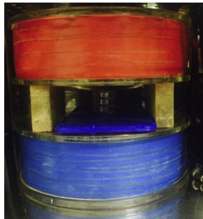
Fig. 1. Image of the EMF stimulation model in CO 2 incubator. We used continuous pulsed EMFs (2 mT) for experiments.
