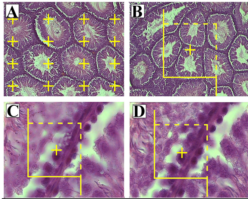
Figure 2: Application of stereological techniques. Point-counting technique to estimate the volume density of the structures (A). Estimation of the length density of the seminiferous tubules by unbiased counting frame (B). Optical disector technique used to estimate the numerical density of the different cells (C and D).
