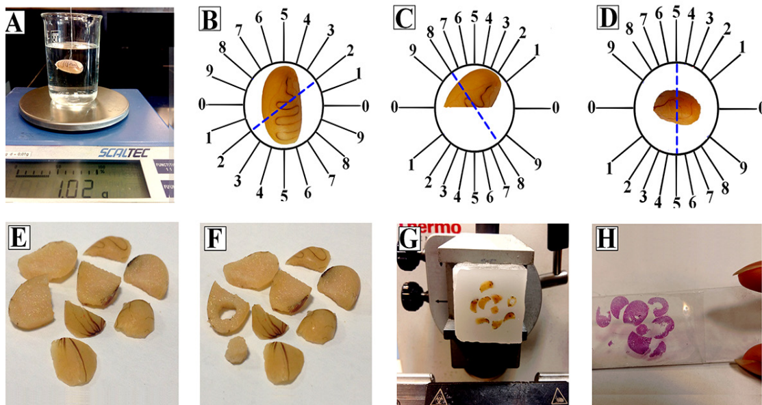
Figure 1: Application of stereological techniques. Determining testis volume according to the Scherle’s method and immersion method (A). Obtaining uniform isotropic tissue sections according to the orientator method (B, C and D). Obtaining a collection of isotropic uniform random sections (E). Punching out a circle through a random slice (F). Embedding and sectioning (G). Tissue slide preparation (H).
