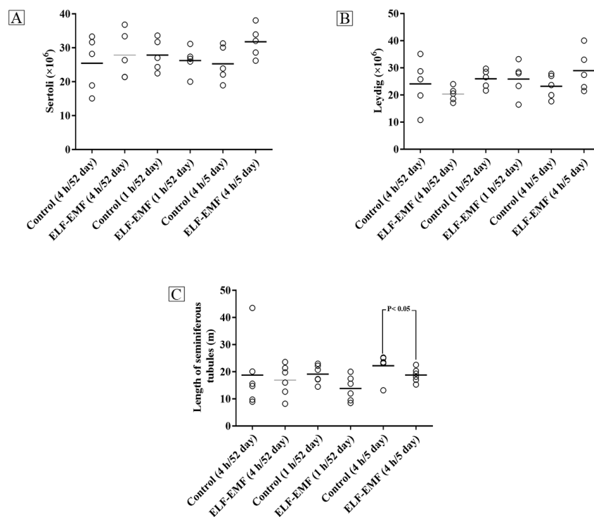
Figure 5: The aligned dot plot of the number of the sertoli (A), and Leydig cells (B) and length of seminiferous tubules (C).
